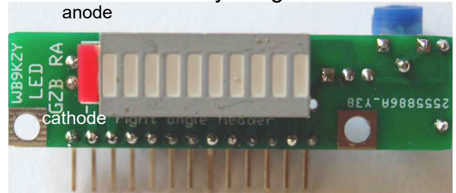
Front view: LED array daughter board
