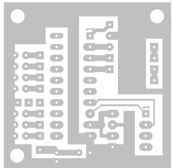
Bottom view of circuit board
