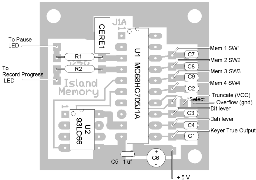
Parts Placement Diagram top view of circuit board
