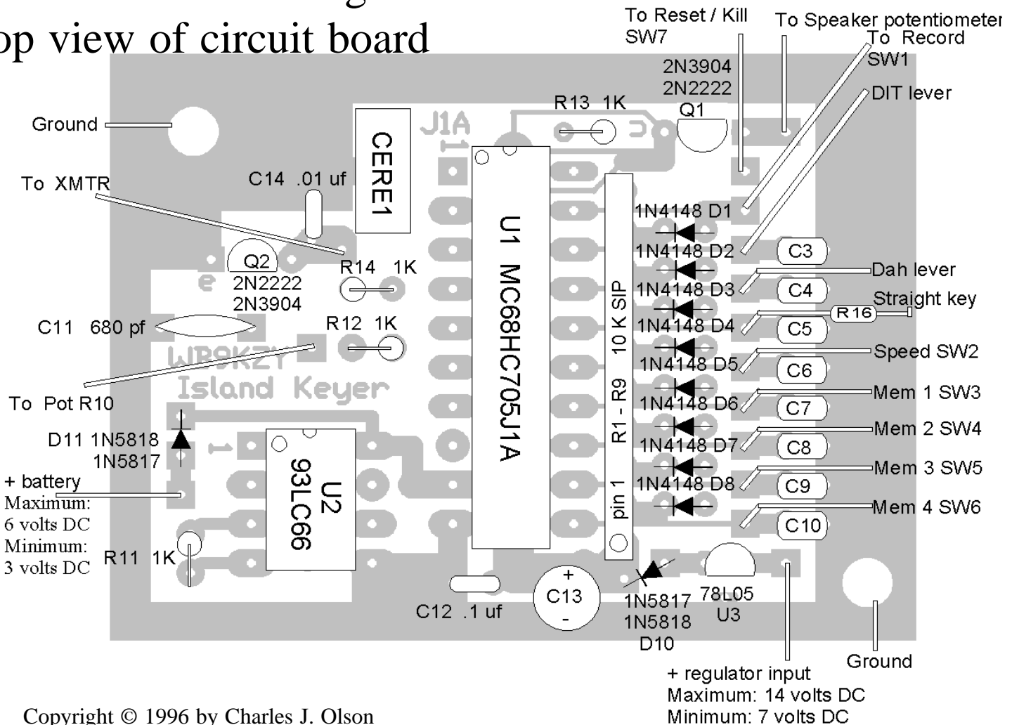
The Island Keyer (WB9KZY Keyer) 1/9/97
