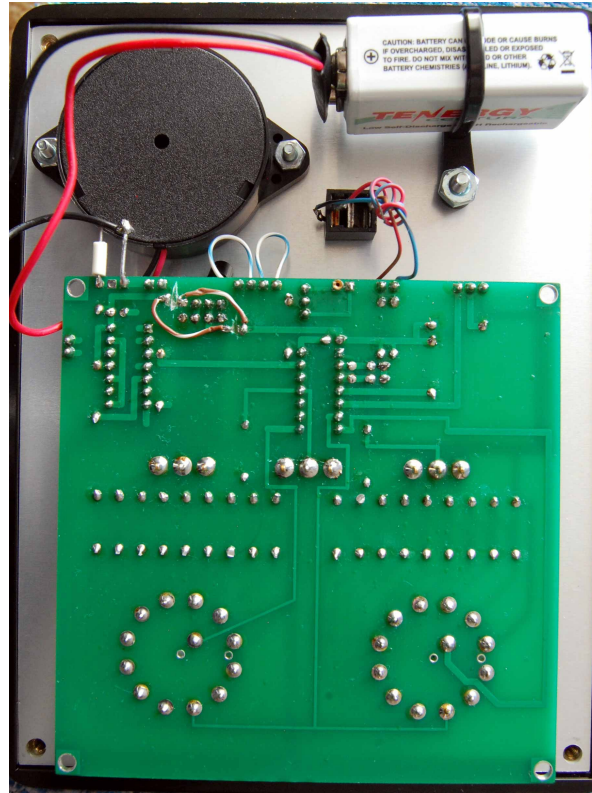
Connections made and board attached
