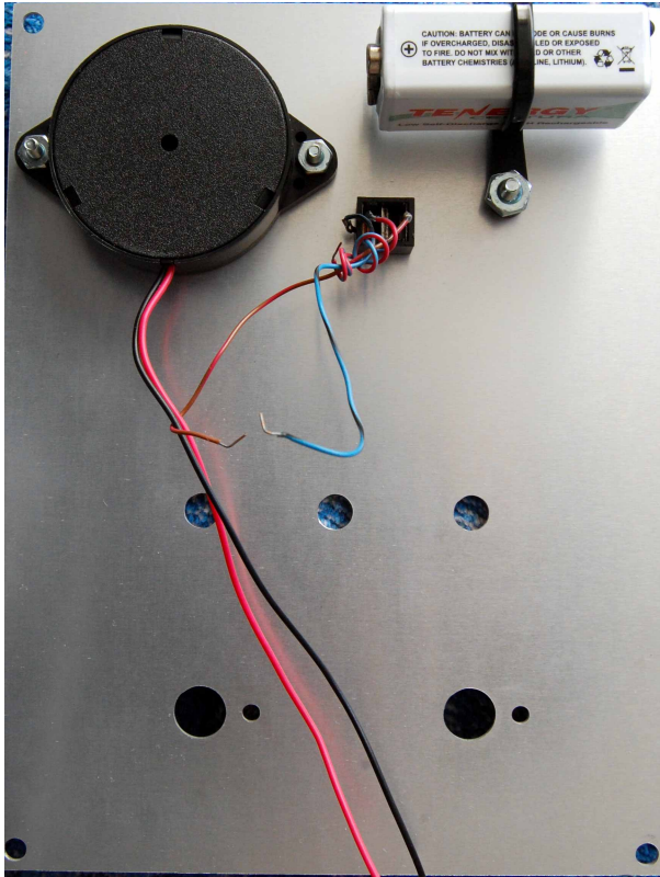
Piezo, jack and battery holder cable tie in place
