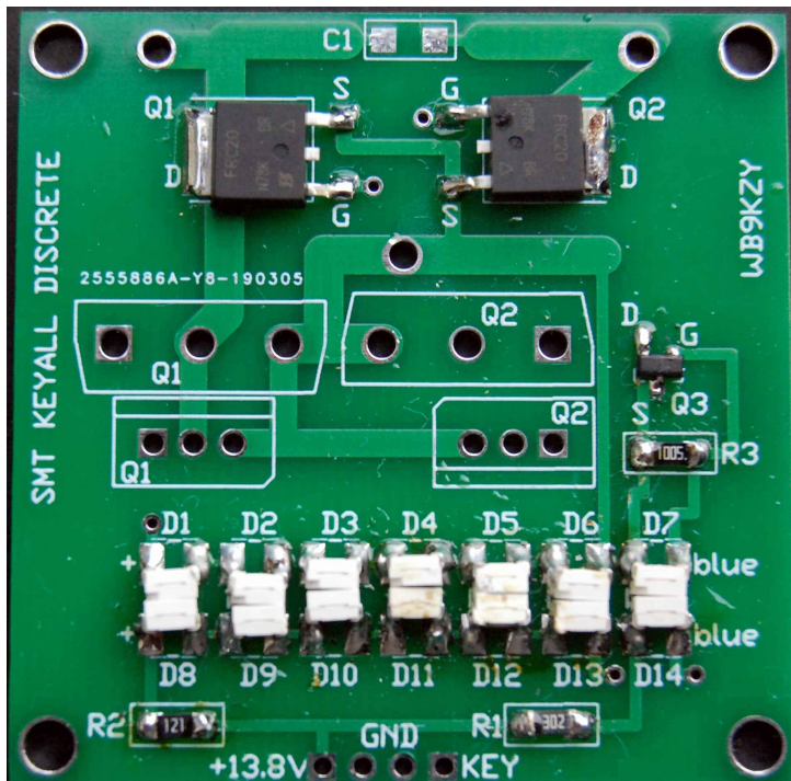
Circuit board Top view:
