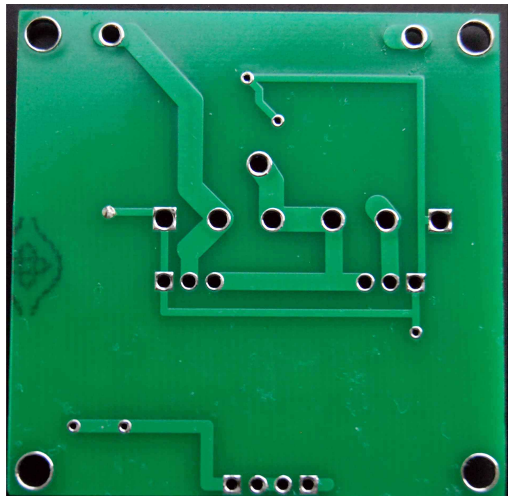
Circuit board Bottom view:
